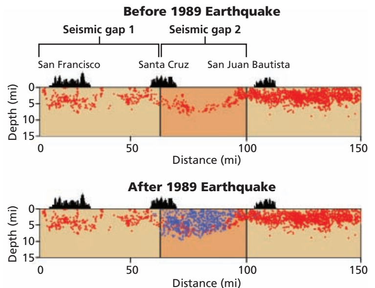
Figure 3 Each red dot in the cross sections of the San Andreas Fault represents an earthquake or aftershock before the 1989 Loma Prieta earthquake. Note how seismic gap 2 was filled by the 1989 earthquake and its aftershocks, which are represented by the blue dots.
