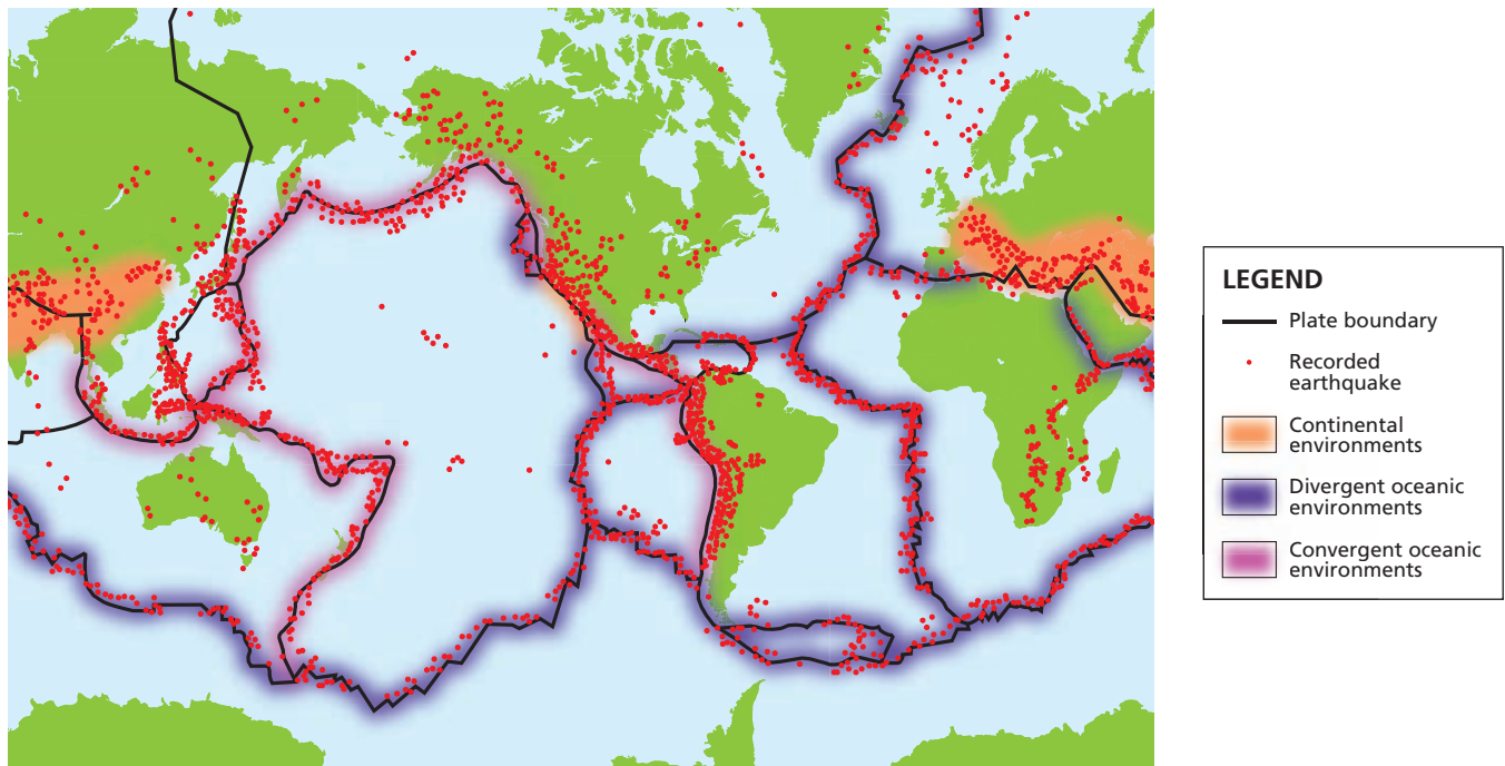
Figure 5 Earthquakes are the result of tectonic stresses in Earth's crust and occur in three main tectonic environments: mid-ocean ridges, subduction zones, and continental collisions.
