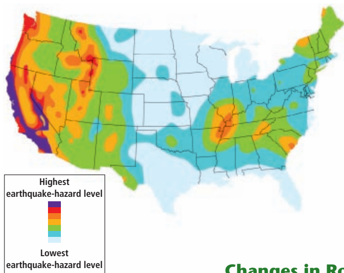
Figure 4 California, which has experienced severe earthquakes recently, has the highest earthquake-hazard level in the contiguous United States.
